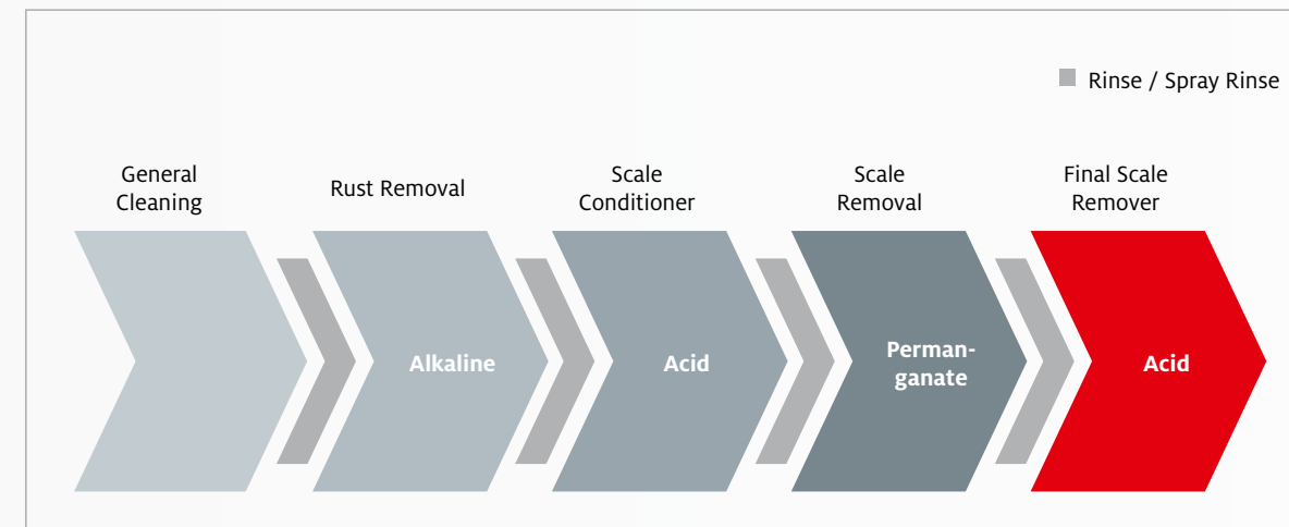
Engine Overhaul Process
